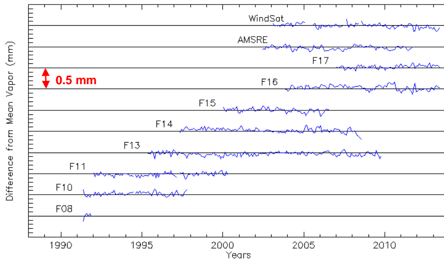
Figure 3: Agreement of TPW measurements from 10 microwave radiometers. The average difference is less than 0.1 mm (kg/m 2 )
