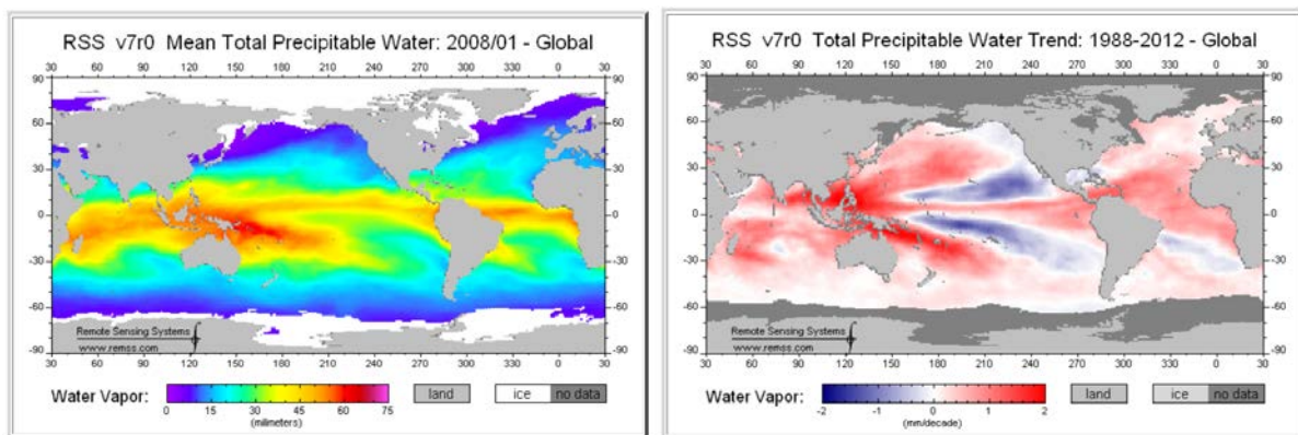
Figure 2: Example of the mean TPW map for January 2008 and the Global TPW trend map for 1988 - 2012.
