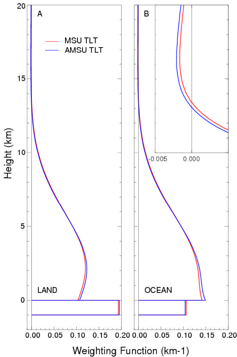
Fig. 3. TLT temperature weighting functions as a function of altitude for MSU and AMSU. As in Fig. 2 the rectangle at the bottom of each panel represents the weight due to surface emission. (A) Weighting functions over land. (B) Weighting functions over ocean. In the inset, we show the two weighting functions on an expanded scale for high altitude.
