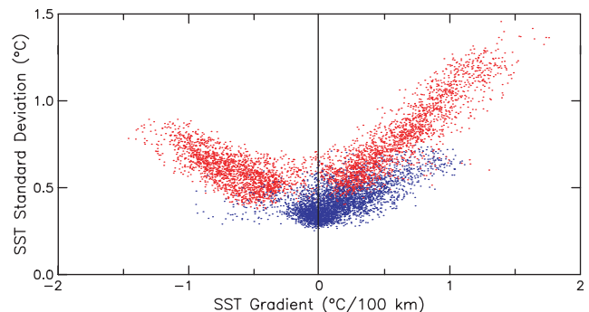
Plate 4. Scatter plot comparison between 50-day high-pass filtered SST and \partial\bar{T}/\partial y for the region 110^{\circ}\text{W} – 160^{\circ}\text{W} , 5^{\circ}\text{S} – 5^{\circ}\text{N} in the Pacific (red dots) and the region 0 – 60^{\circ}\text{W} , 5^{\circ}\text{S} – 5^{\circ}\text{N} in the Atlantic (blue dots).
